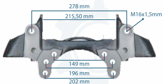
111327 CALIPER CARRIER SCHMITZ K108001K50
