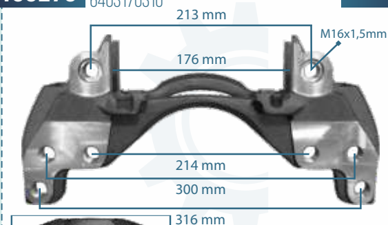
133279 CALIPER CARRIER MAXX17 LEFT 6403170310
