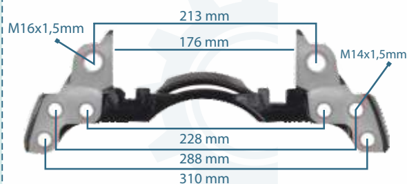
133126 CALIPER CARRIER 17.5" RIGHT
