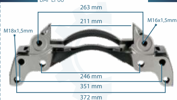
133262 CALIPER CARRIER PAN 19 RIGHT DAF LF55
