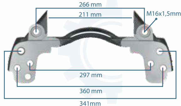
111332 CALIPER CARRIER LEFT IVECO K002313
