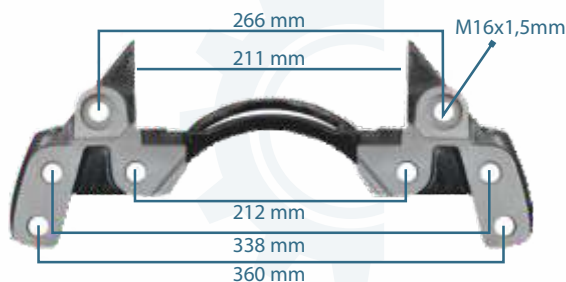
111200 CALIPER CARRIER BUS 19.5"
