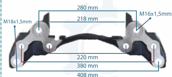
133127 CALIPER CARRIER MAXX 22 LEFT
