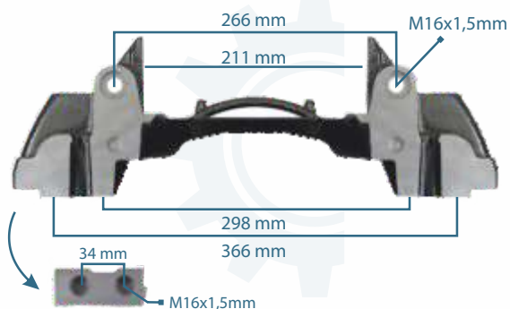
111315 CALIPER CARRIER 22.5" K012619 - Z006715 - 2379697
