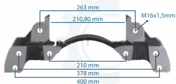
133178 CALIPER CARRIER PAN22 LEFT
