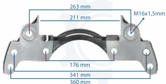
133219 CALIPER CARRIER 19.5" LEFT 40195037
