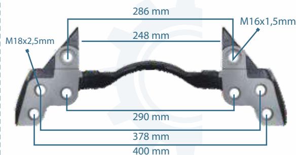
111262 CALIPER CARRIER 22.5" K011479 - 1689314 - Z006590
