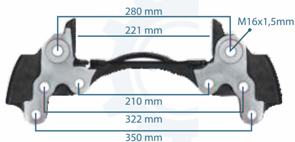
133163 CALIPER CARRIER MB AROCS (LEFT) 000 423 2306 - 640 915 744 4
