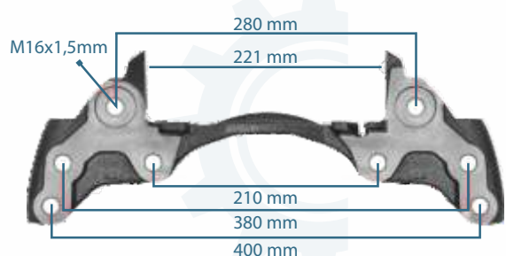
133183 CALIPER CARRIER MB AROC FRONT RIGHT A0004216406 - 6409157434
