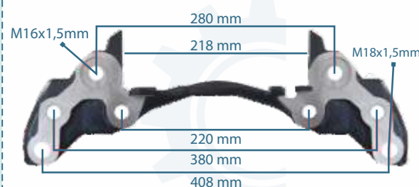
133128 CALIPER CARRIER MAXX 22 RIGHT
