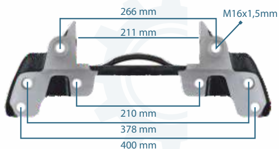
111317 CALIPER CARRIER 22.5" SK7 K004099 - Z012024 - 2121600
