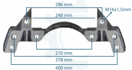
111229 CALIPER CARRIER 22.5" FRONT (LEFT&RIGHT)
