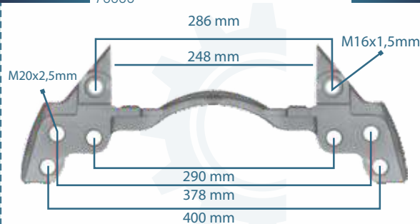
111334 CALIPER CARRIER 22.5" DAF 73355
