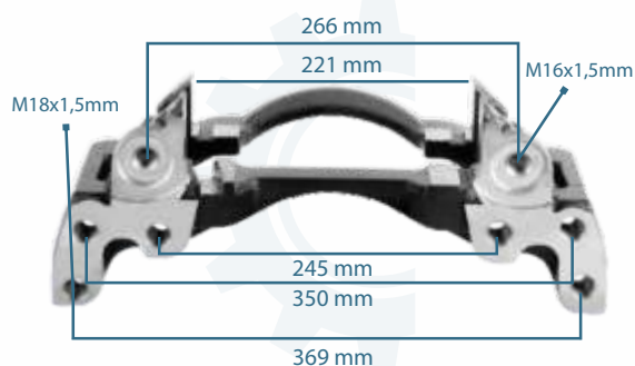
133180 CALIPER CARRIER MAXX19 LEFT
