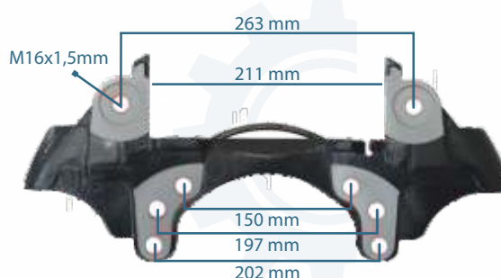
133222 CALIPER CARRIER RIGHT VALX AXLE 6402250310
