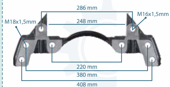
111220 CALIPER CARRIER MAN TGA
