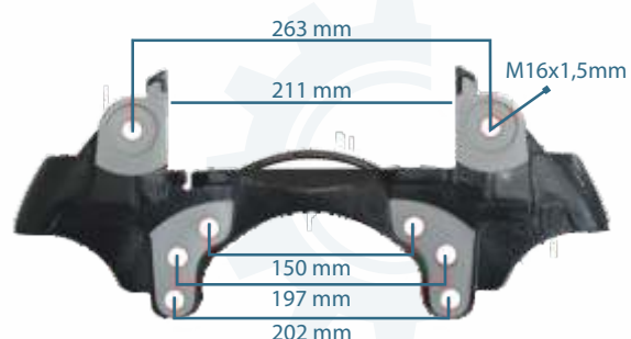
133221 CALIPER CARRIER LEFT VALX AXLE 6402250300
