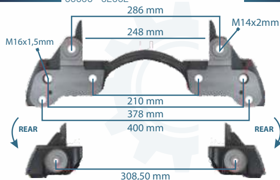
144133 CALIPER CARRIER 22.5" LEFT & RIGHT 90636 - 92502
