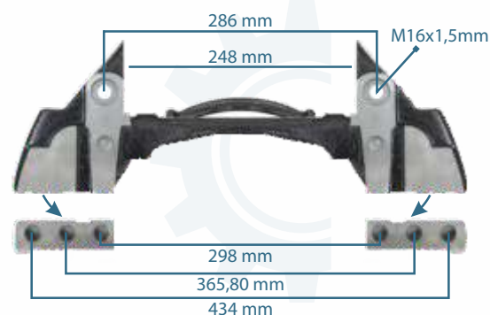
111318 CALIPER CARRIER 22.5" K004680 - 2379696 - 01.303.88.57.0
