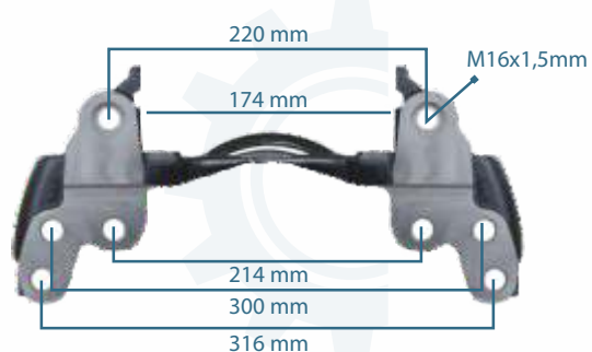
111203 CALIPER CARRIER 17.5"
