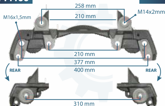
144136 CALIPER CARRIER GIGANT AXLE
