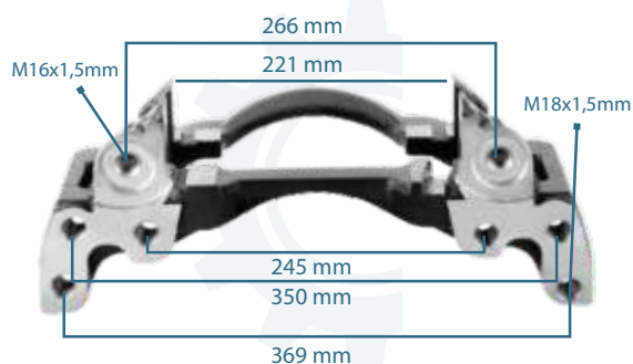
133181 CALIPER CARRIER MAXX19 RIGHT
