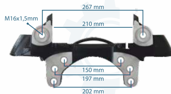
133224 CALIPER CARRIER RIGHT SCHMITZ 6402227406 D1-6J20
