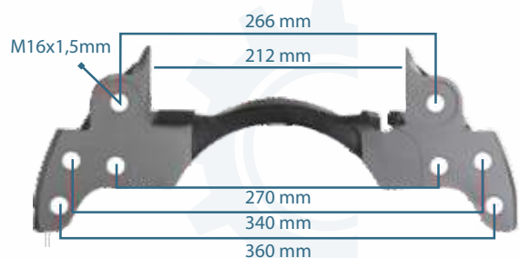
133218 CALIPER CARRIER PAN 19 RIGHT
