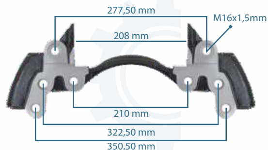
111263 CALIPER CARRIER SL7 REAR 22,5" (LEFT-RIGHT) K052379K50 - Z025197 - 000 423 1006
