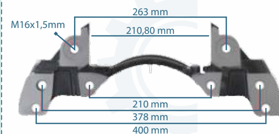
133179 CALIPER CARRIER PAN22 RIGHT
