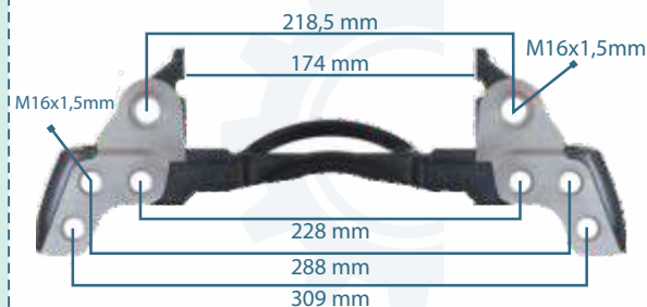
111201 CALIPER CARRIER MAN 12-160
