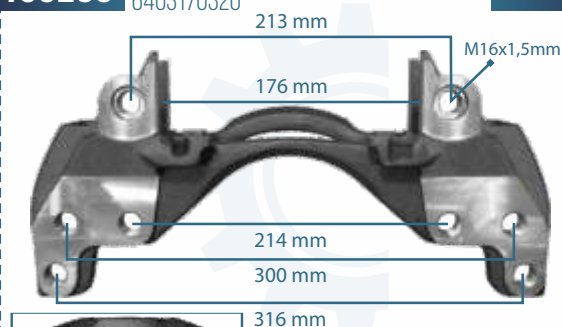
133280 CALIPER CARRIER MAXX17 RIGHT 6403170320
