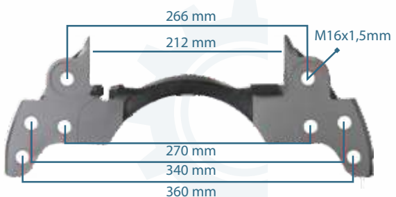
133217 CALIPER CARRIER PAN 19 LEFT
