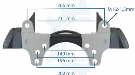
111264 CALIPER CARRIER SCHMITZ TRAILER K007475 - Z000968
