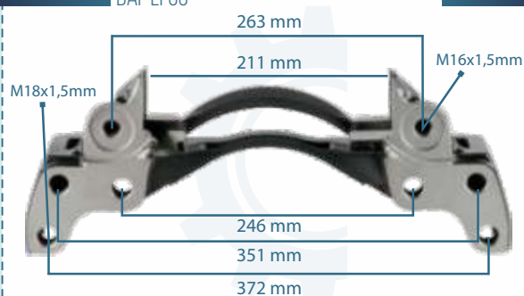
133261 CALIPER CARRIER PAN 19 LEFT DAF LF55
