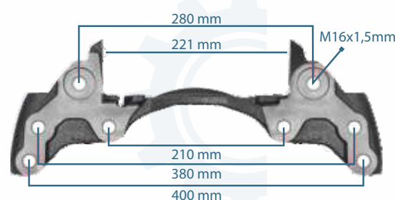
133182 CALIPER CARRIER MB AROC FRONT LEFT A0004216506 - 6409157424
