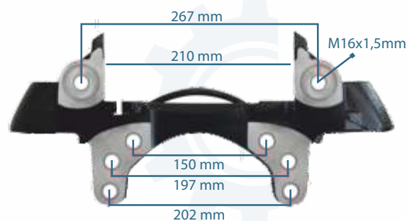
133223 CALIPER CARRIER LEFT SCHMITZ 6402227406 D3-6K25
