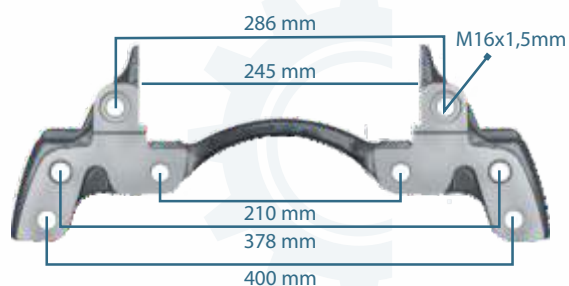
111221 CALIPER CARRIER MB4140
