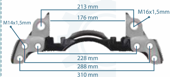
133125 CALIPER CARRIER 17.5" LEFT
