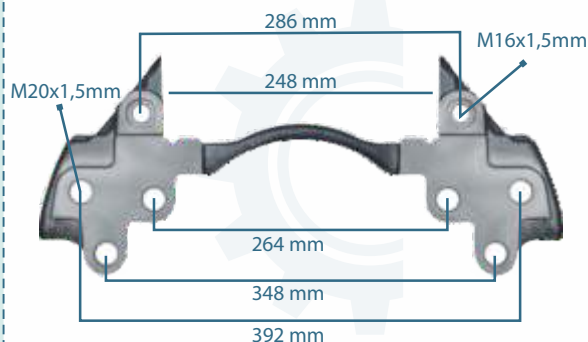
111202 CALIPER CARRIER 22.5"
