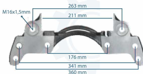
133220 CALIPER CARRIER 19.5" RIGHT 40195038
